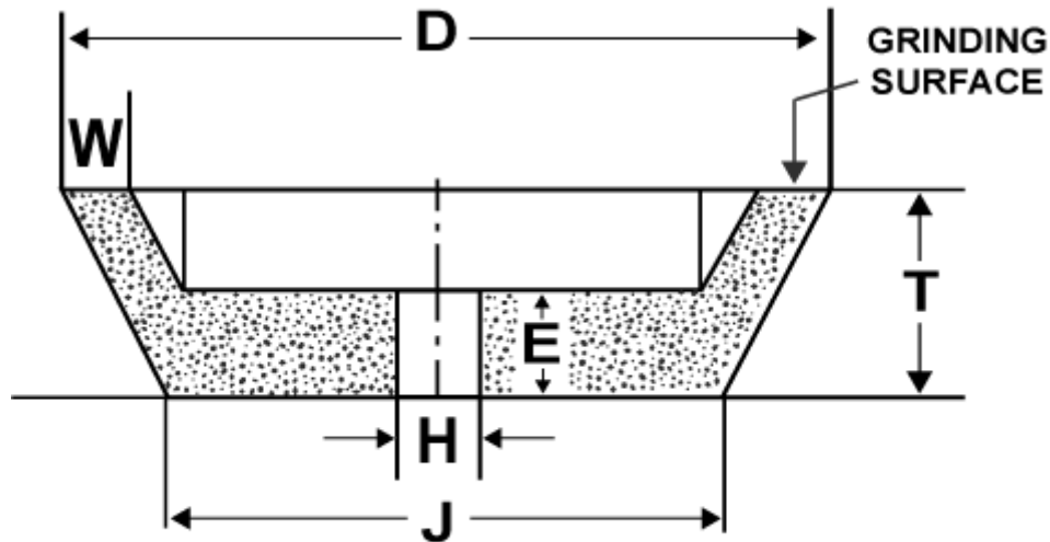
TYPE 11 - FLARING CUP WHEEL
