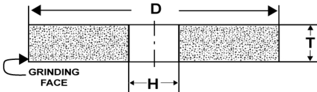
TYPE 1 - STRAIGHT WHEELS
